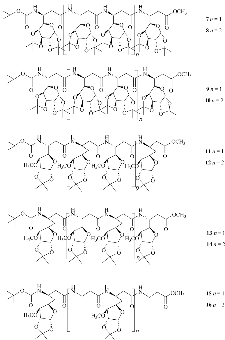
Figure 2. Structures of peptides 7–16.
