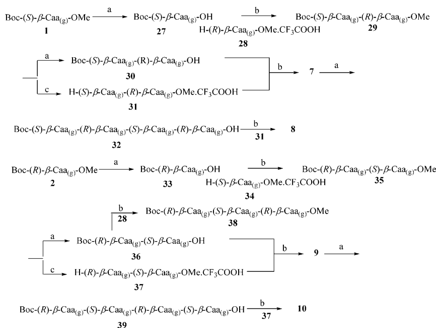
Scheme 3. Synthesis of peptides 7 – 10 containing 1 and 2 . a) 4\text{N NaOH} , \text{CH}_3\text{OH} , 0^\circ\text{C} –RT; b) \text{HOBt} (1.2 equiv), \text{EDCI} (1.2 equiv), \text{DIPEA} (1.5 equiv), dry \text{CH}_2\text{Cl}_2 , 0^\circ\text{C} –RT; c) \text{CF}_3\text{COOH} , dry \text{CH}_2\text{Cl}_2 , 0^\circ\text{C} –RT.
