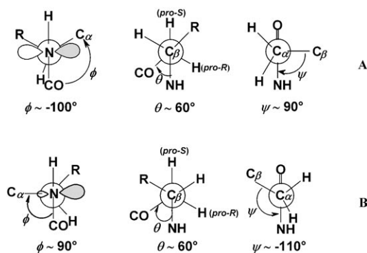
Figure 4. Schematic Newman projections showing the orientation of substituents in 10/12-right-handed helix for the ideal values of torsional angles \phi , \theta and \psi . [5b] view along the backbone atoms in: (A) (R) - \beta -Caa (g) and (B) (S) - \beta -Caa (g) .
