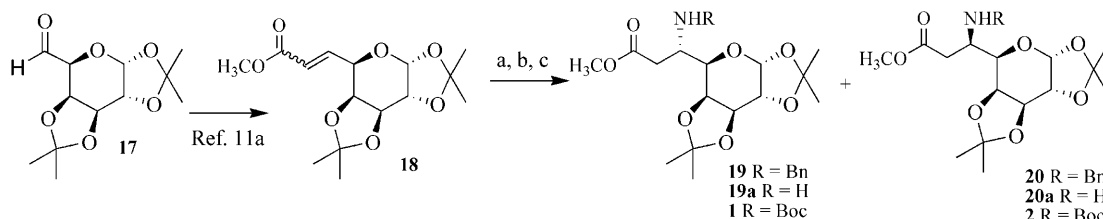
Scheme 1. Synthesis of amino acids 1 and 2 . a) \text{BnNH}_2 , RT, 12h; b) \text{H}_2 , 10% Pd-C, \text{CH}_3\text{OH} , RT, 12h; c) (\text{Boc})_2\text{O} , \text{Et}_3\text{N} , THF, 0^\circ\text{C} –RT, 2h.
