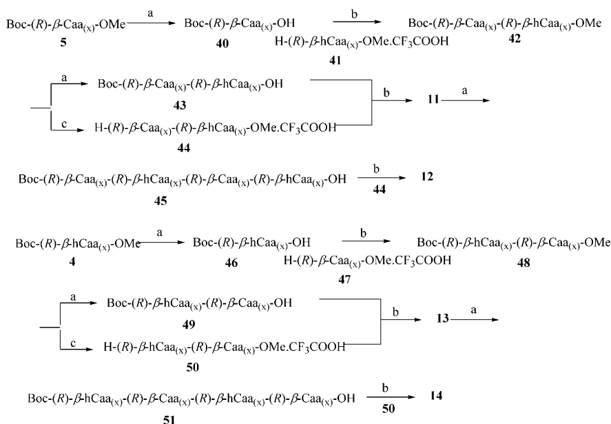
Scheme 4. Synthesis of peptides 11–14 having alternating 4 and 5 . a) 4N NaOH, CH 3 OH, 0°C–RT; b) HOBT (1.2 equiv), EDCI (1.2 equiv), DIPEA (1.5 equiv), dry CH 2 Cl 2 , 0°C–RT; c) CF 3 COOH, dry CH 2 Cl 2 , 0°C–RT.
