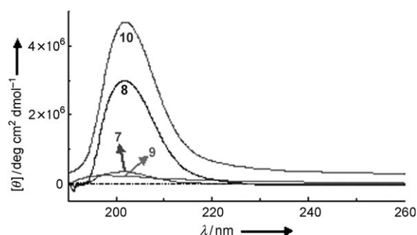
Figure 9. CD spectra of 7–10 .
