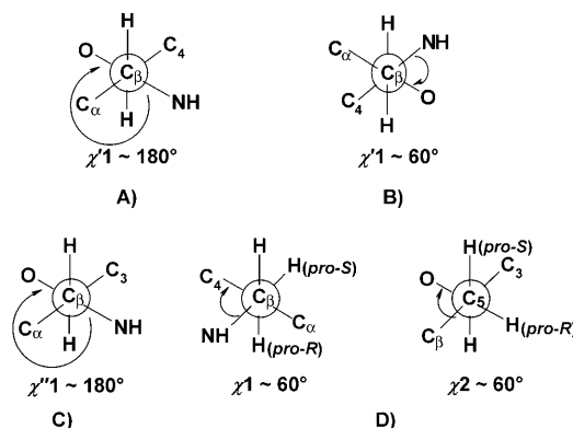
Figure 8. Newman projections showing the orientations of various substituents for the predominant conformers about the C–C bonds, appending the sugar side chains to the peptide backbone. About C \beta –C \gamma ( \chi'_1 ) (A) for ( R )- \beta -Caa (g) and (B) for ( S )- \beta -Caa (g) ; (C) About C \beta –C _4 ( \chi''_1 ) for ( R )- \beta -Caa (x) ; (D) About C \beta –C _5 ( \chi_1 ) and C _5 –C _4 ( \chi_2 ) for ( R )- \beta -hCaa (x) .
