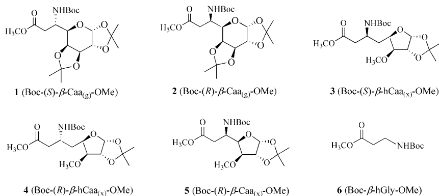
Figure 1. Structures of \beta -amino acids 1–6 .
